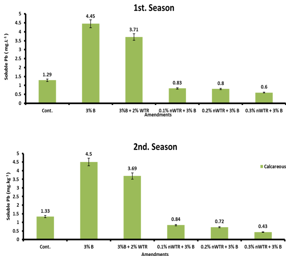
Fig.11. Impact of nWTRs on the concentration of soluble lead in the soil solution of calcareous soil treated with biosolids, WTRs, and nWTRs
