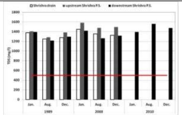
Fig.4. The relation between TDS and time of sampling of Shrishra drain, upstream Shrishra P.S. and downstream Shrishra P.S.
