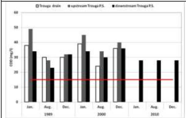
Fig.11. The relation between COD and time of sampling of Trouga drain, upstream Trouga P.S. and downstream Trouga P.S.
