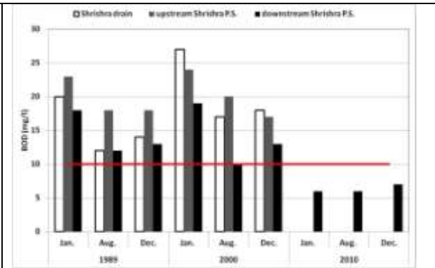
Fig.16. The relation between BOD and time of sampling of Shrishra drain, upstream Shrishra P.S. and downstream Shrishra P.S.
