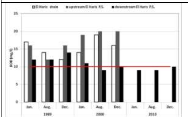
Fig.19. The relation between BOD and time of sampling of El Haris drain, upstream El Haris P.S. and downstream El Haris P.S.
