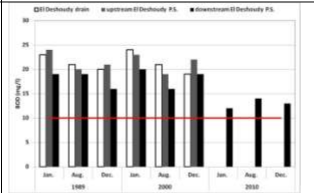
Fig.18. The relation between BOD and time of sampling of El Deshody drain, upstream El Deshody P.S. and downstream El Deshody P.S.
