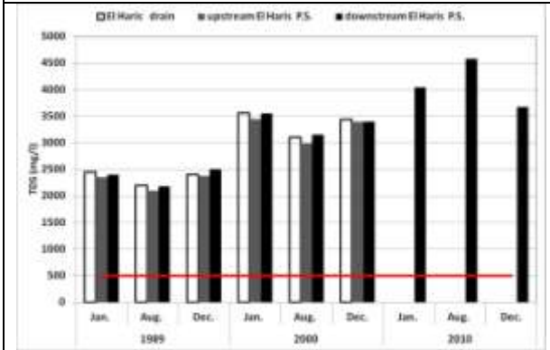
Fig.7. The relation between TDS and time of sampling of El Haris drain, upstream El Haris P.S. and downstream El Haris P.S.
