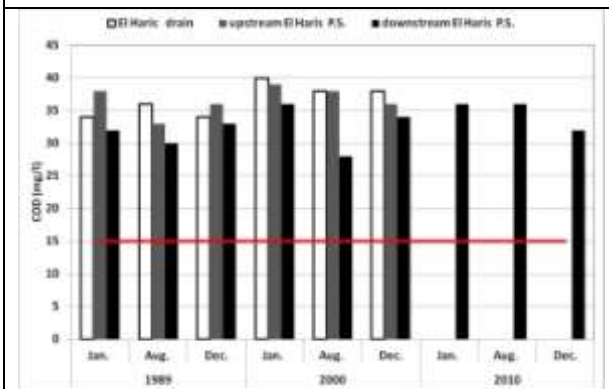
Fig.13. The relation between COD and time of sampling of El Haris drain, upstream El Haris P.S. and downstream El Haris P.S.
