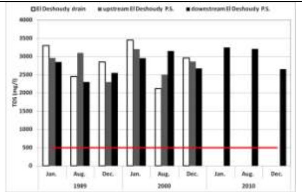
Fig.6. The relation between TDS and time of sampling of El Deshoudy drain, upstream El Deshoudy P.S. and downstream El Deshoudy P.S.
