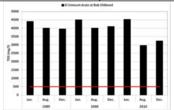
Fig.8. The relation between TDS and time of sampling of El Umoum drain at Bab ElAbeed.
