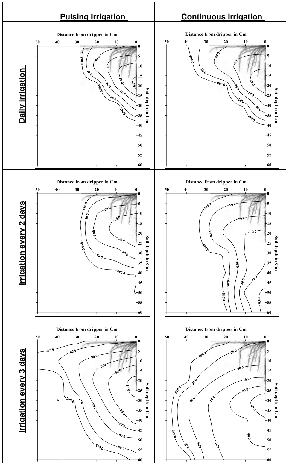
Figure 3. Redistribution of volumetric soil moisture content for both pulsing and continuous irrigation before irrigation at peak of water consumption for the crop (mid stage)
